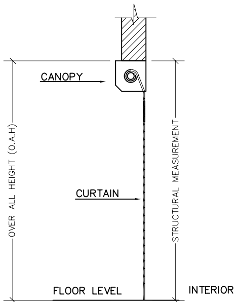
RECESS FIT
